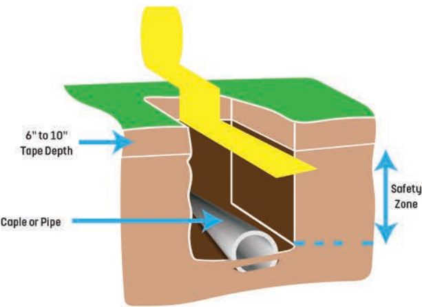
Underground warning tape is normally installed a specified distance directly above the service line so that any future excavators will be aware of the cable or pipeline further below.
